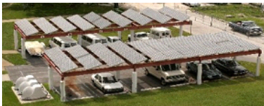
CERC's 20,000 watt solar / electric charging station at the USF in Tampa.
