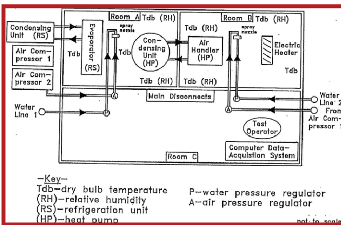
CERC's ASHRAE Standard test facility on the University of South Florida (Tampa) campus.
